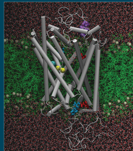
Snapshot from a full-atomic molecular dynamics simulation of a dopamine transporter (grey cylinders) embedded in a lipid bilayer (green) and water molecules (red/grey) on both the extracellular and intracellular regions. (Courtesy of Dr M H Cheng).
